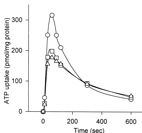
Fig. 5. trans -Stimulation of ATP transport by ADP. ADP- and AMP-preloaded proteoliposomes were constructed using reconstitution buffer containing 200 \mu\text{M} of ADP and ATP as described in Section 2. Time-course of ATP transport activity is displayed for ADP( \circ )-, AMP( \triangle )-preloaded RER proteoliposomes and control ( \square ). Data points represent the mean values for three experiments.
